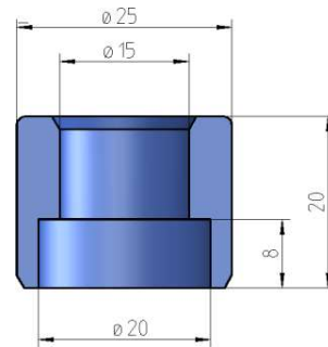
Spannzangenhülse Collet chuck bushing 05-002-923
